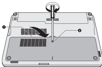
Figure 3-12 Seating the memory module cover
