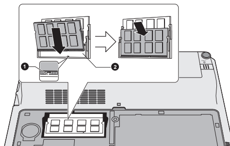
Figure 3-11 Seating the memory module
