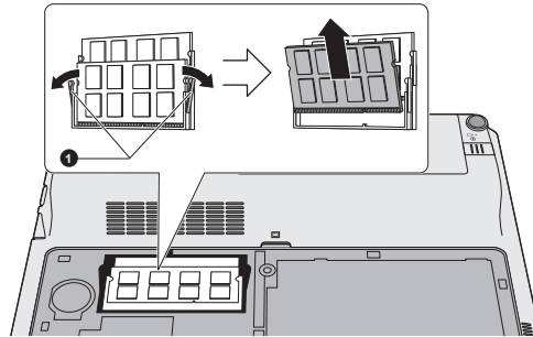
Figure 3-13 Removing the memory module
